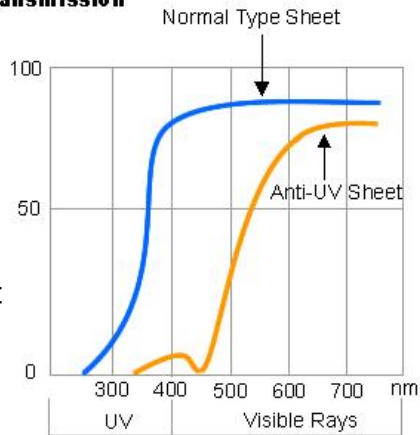
Light Transmission
